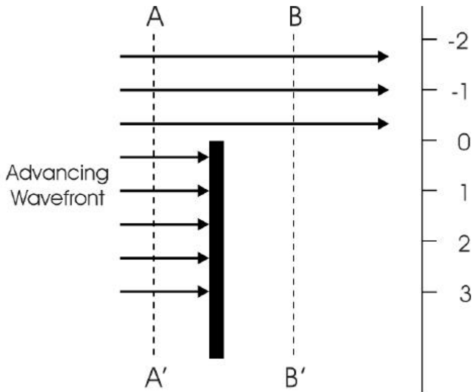
Figure 1 Shadowing of Radio Waves by an Object
